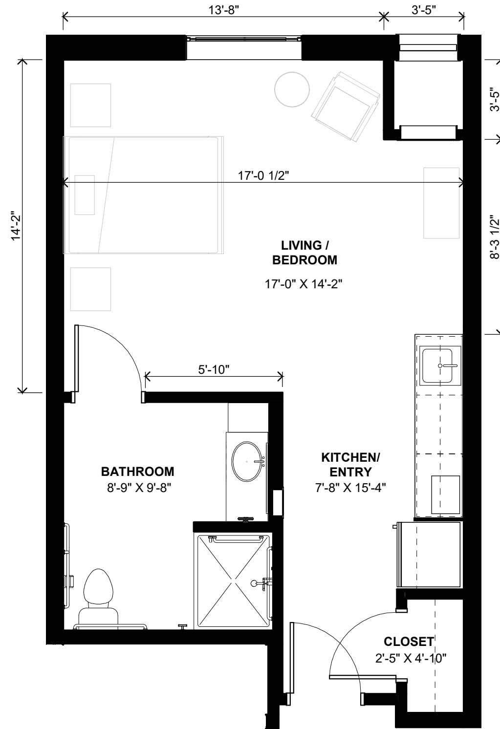
1 UNIT MC1- FLOOR PLAN 1/4" = 1'-0" 0 3' 6'
