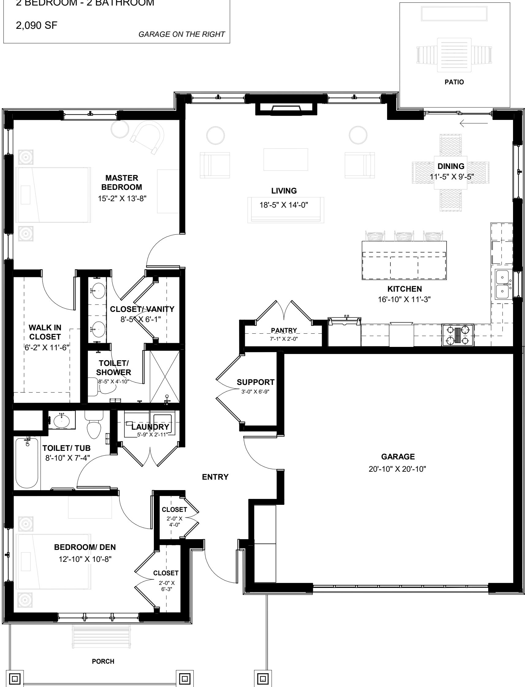
1 TOWNHOUSE - FLOOR PLAN 3/16" = 1'-0"
